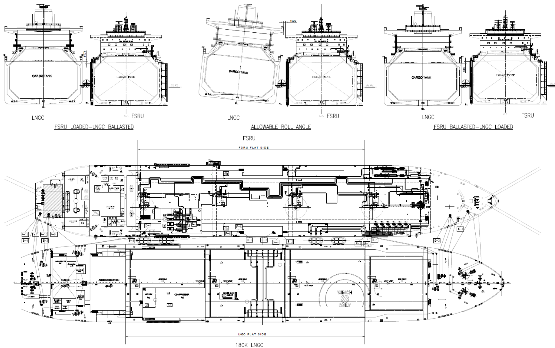
Figure 22 Proposed mooring plan with LNGC up to 180000 LNGC
