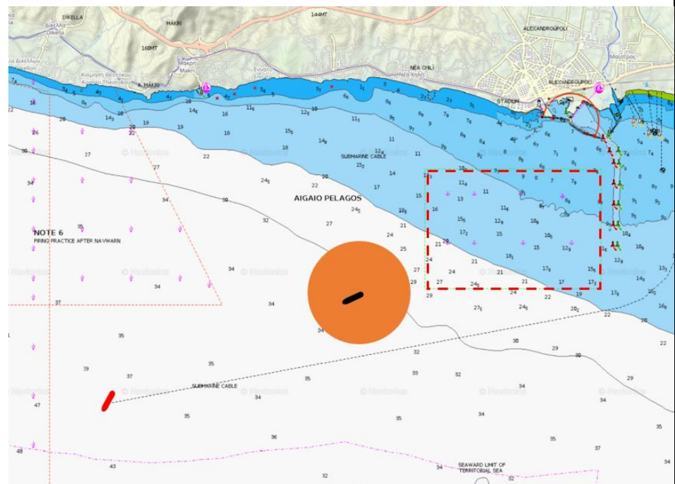
Figure 2 Proposed Pilot boarding area
