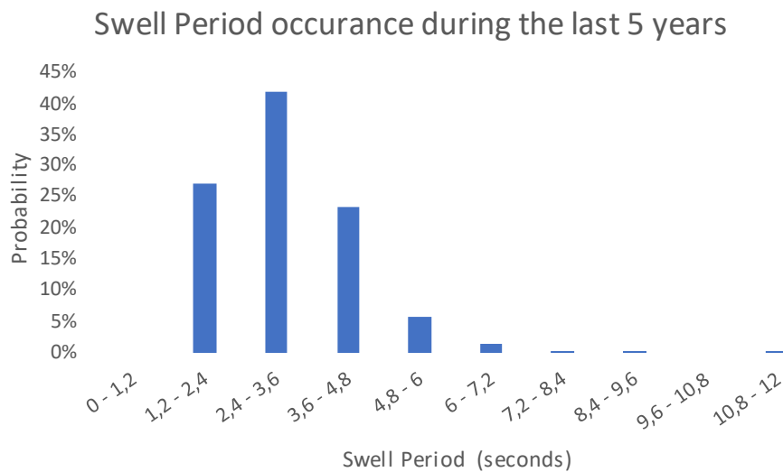
Figure 6 Swell Period - Offshore Alexandroupolis
