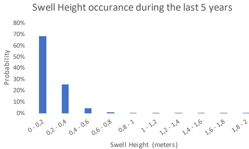
Figure 5 Swell Height – Offshore Alexandroupolis
