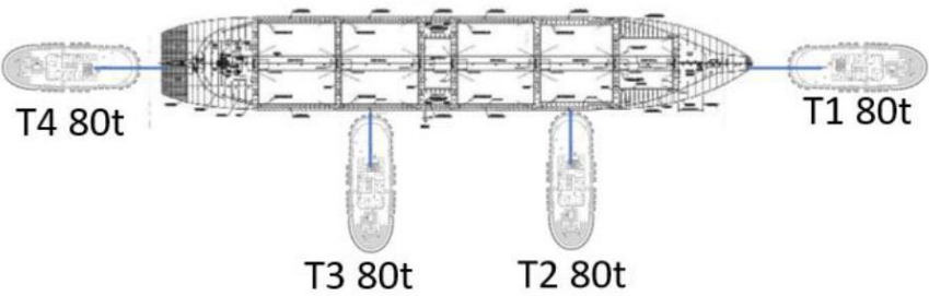
Figure 1 Typical Tug Arrangement
