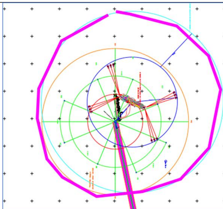
Figure 3 FSRU Exclusion Zone
